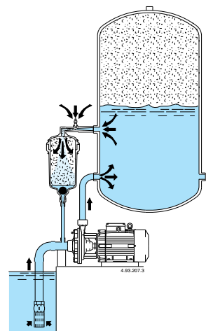
3) The water level in the ARIAMAT drops until the ball valve moves to the bottom of the ARIAMAT closing the hole of the pipe connected to the pump. ARIAMAT is now full of air.
